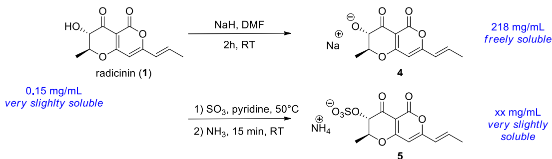
Scheme 2: Alternative radacinin derivatives prepared, and their solubility in water.
