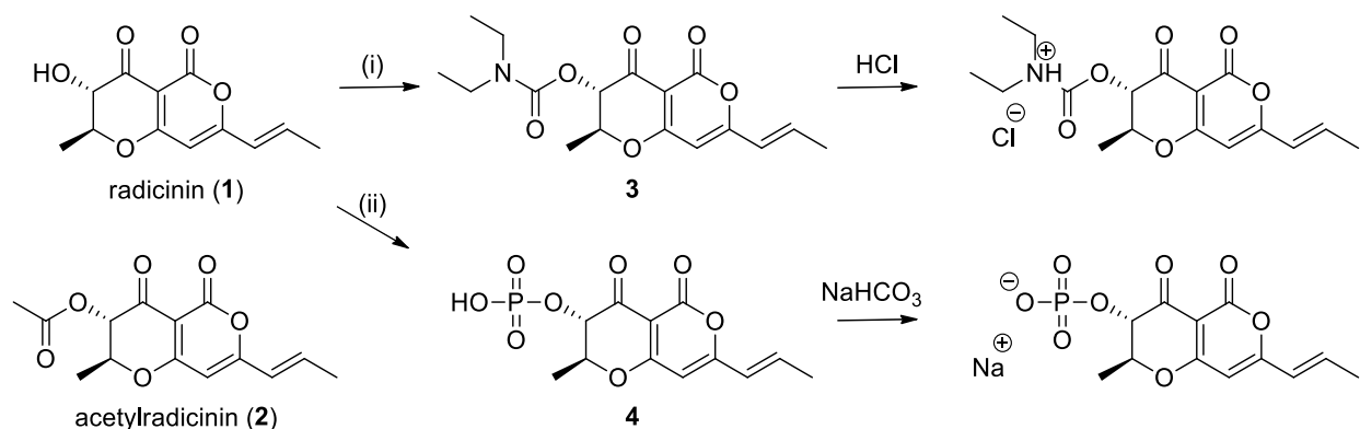
Scheme 1: Xf -inhibitory natural product radicinin (1), and semisynthetic derivatives (2-4). Reagents: (i) N,N -diethylcarbamoyl chloride, triethylamine (Vougianniopoulou et al. 2008). (ii) 1. Cl_3CCN , 2. (n-Bu)_4NH_2PO_4 , CH_3CN , 3. DOWEX 50WX8, NH_4HCO_3 (Lira et al. 2013).
