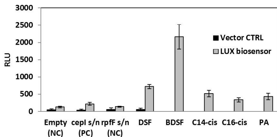
Figure 1. Bioluminescence exhibited by the Burk-DSF biosensor in KB media containing no added DSF (rpfFs/n) or 3 uM DSF (C13), BDSF (C12), Xf DSF1 (C14-cis), Xf DSF2 (C16-cis), or palmitoleic acid (PA).
